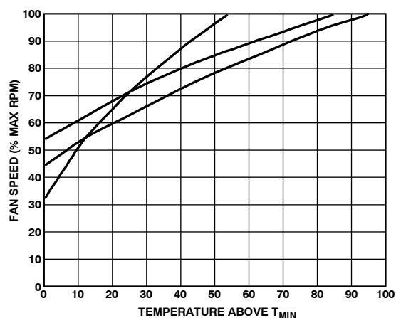
Figure 66. T_{RANGE} and Percentage of Fan Speed Slopes for VRM, Ambient, and CPU Temperature Channels
