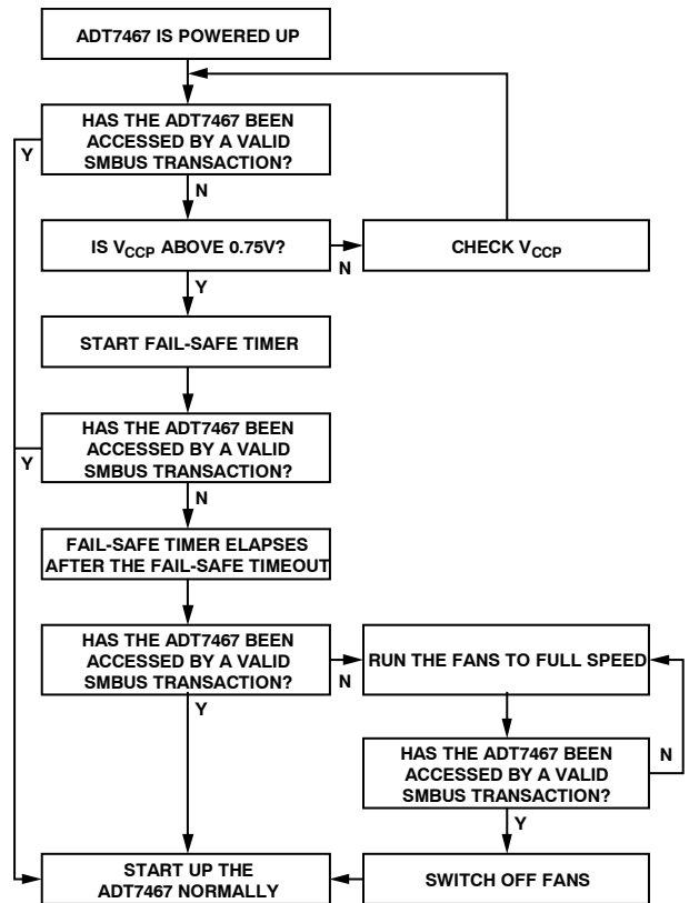
Figure 48. Power-On Flowchart
