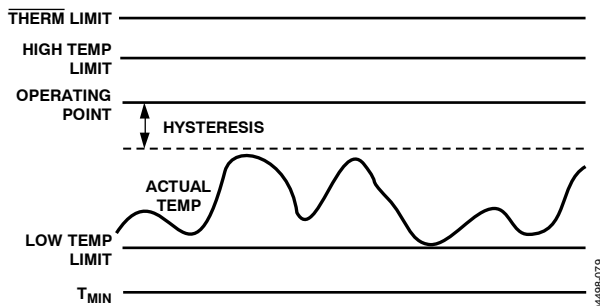
Figure 72. Temperature Between Operating Point and Low Temperature Limit
