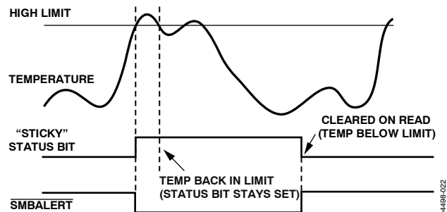
Figure 28. SMBALERT and Status Bit Behavior
