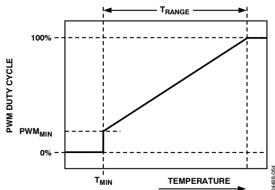
Figure 61. T RANGE Parameter Affects Cooling Slope
