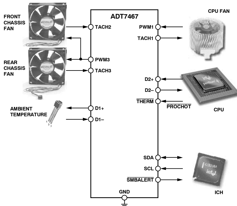
Figure 15. ADT7467 Configuration
