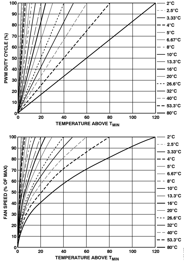
Figure 64. T_{RANGE} vs. Fan Speed Profile
